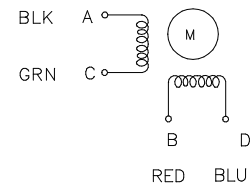
Wiring Diagram
