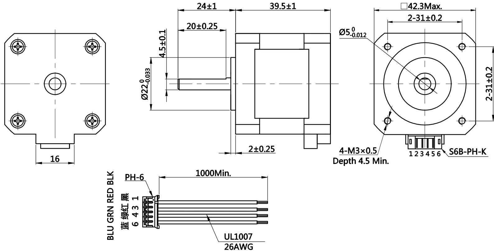
外形图 (DIMENSIONS) unit=mm
